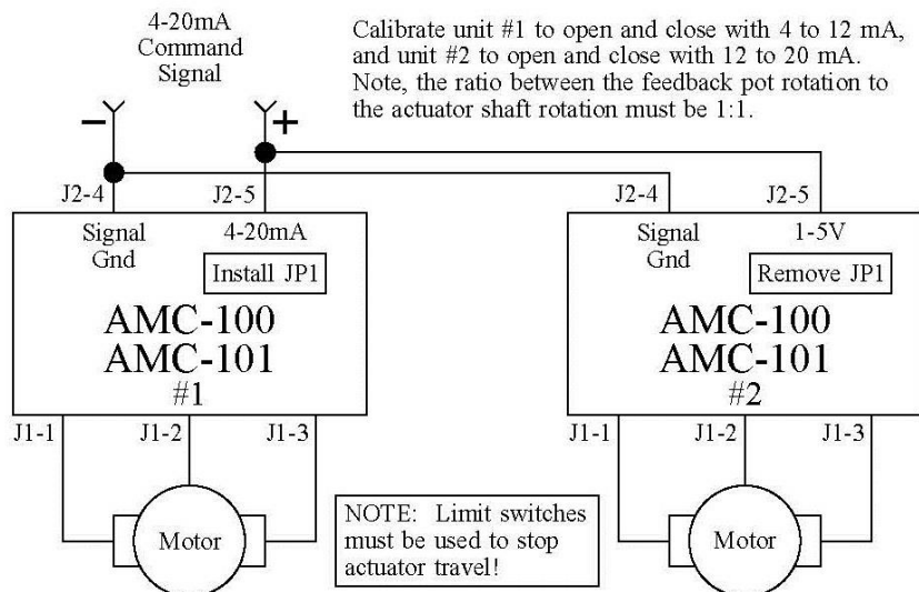
Split range control
